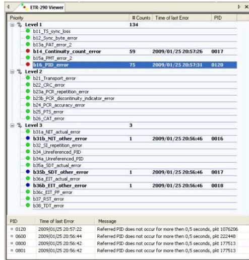
ETR-290 Viewer
