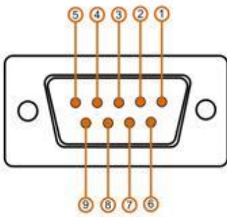
DB-9 Connector (Female) Pin #'s
