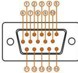
DB-15 Connector (Male) Pin #'s
