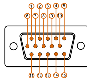
DB-15 Connector (Male) Pin #'s
