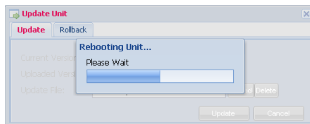
Figure 57: Unit restarting
