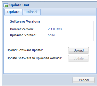
Figure 52: Updating software
