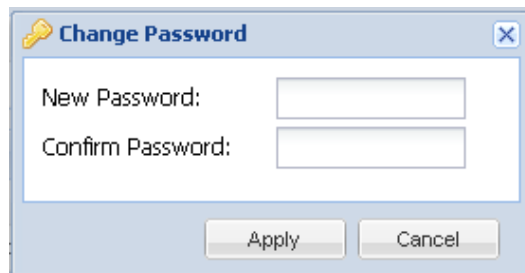
Figure 50: Setting password
