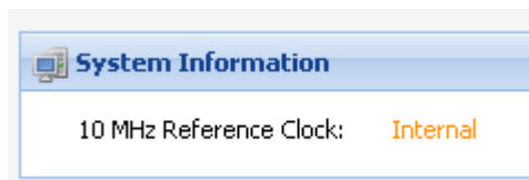
Figure 60: Reference clock
