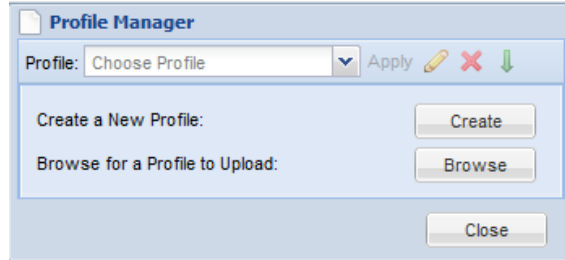
Figure 49: Profile Manager
