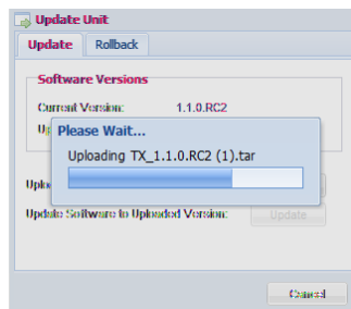
Figure 53: Uploading file
