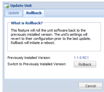
Figure 58: Software rollback
