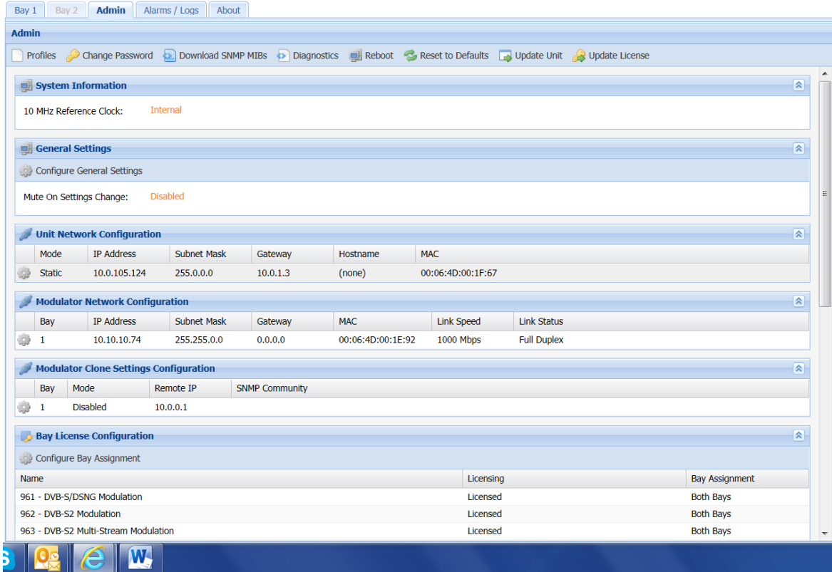
Figure 47: Admin tab
