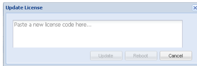
Figure 59: Update License
