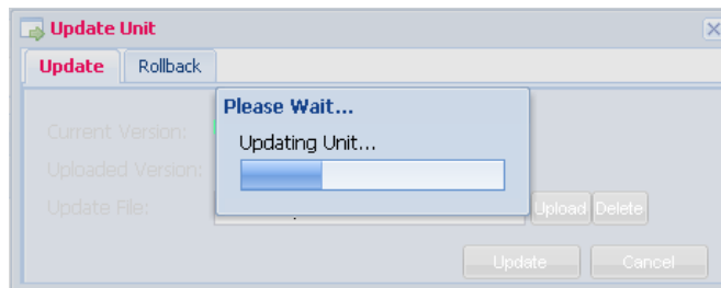
Figure 56: Updating unit
