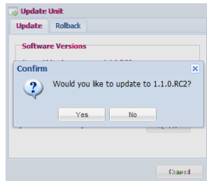
Figure 55: Update confirmation
