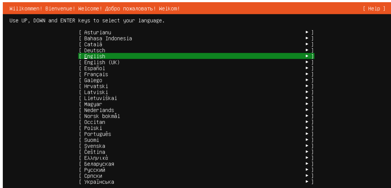
Figure 3.1: Welcoming screen
